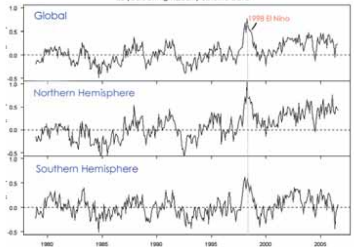
Half the globe is not warming 28 years of High Quality Satellite Data
