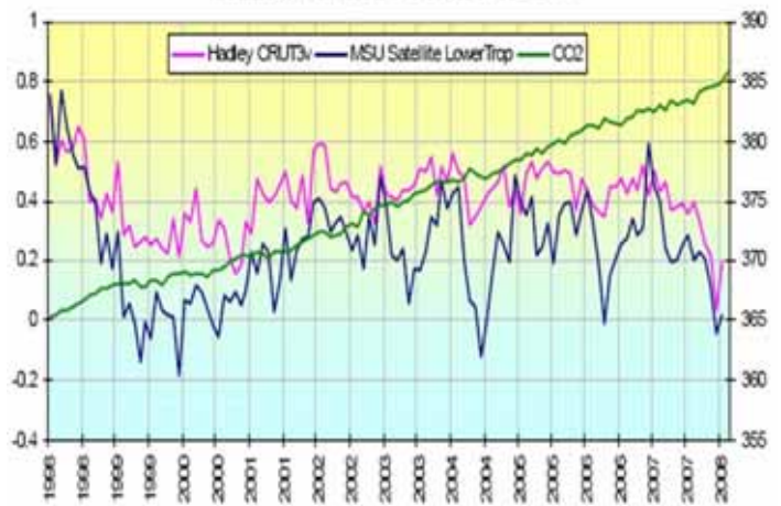
Hadley and MSU Temps vs CO2
