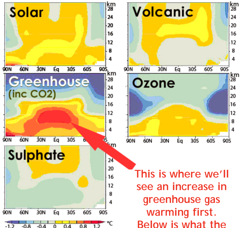
Source: IPCC 2007, p 675, based on Santer et al 2003. See also IPCC 2007, Appendix 9C.
